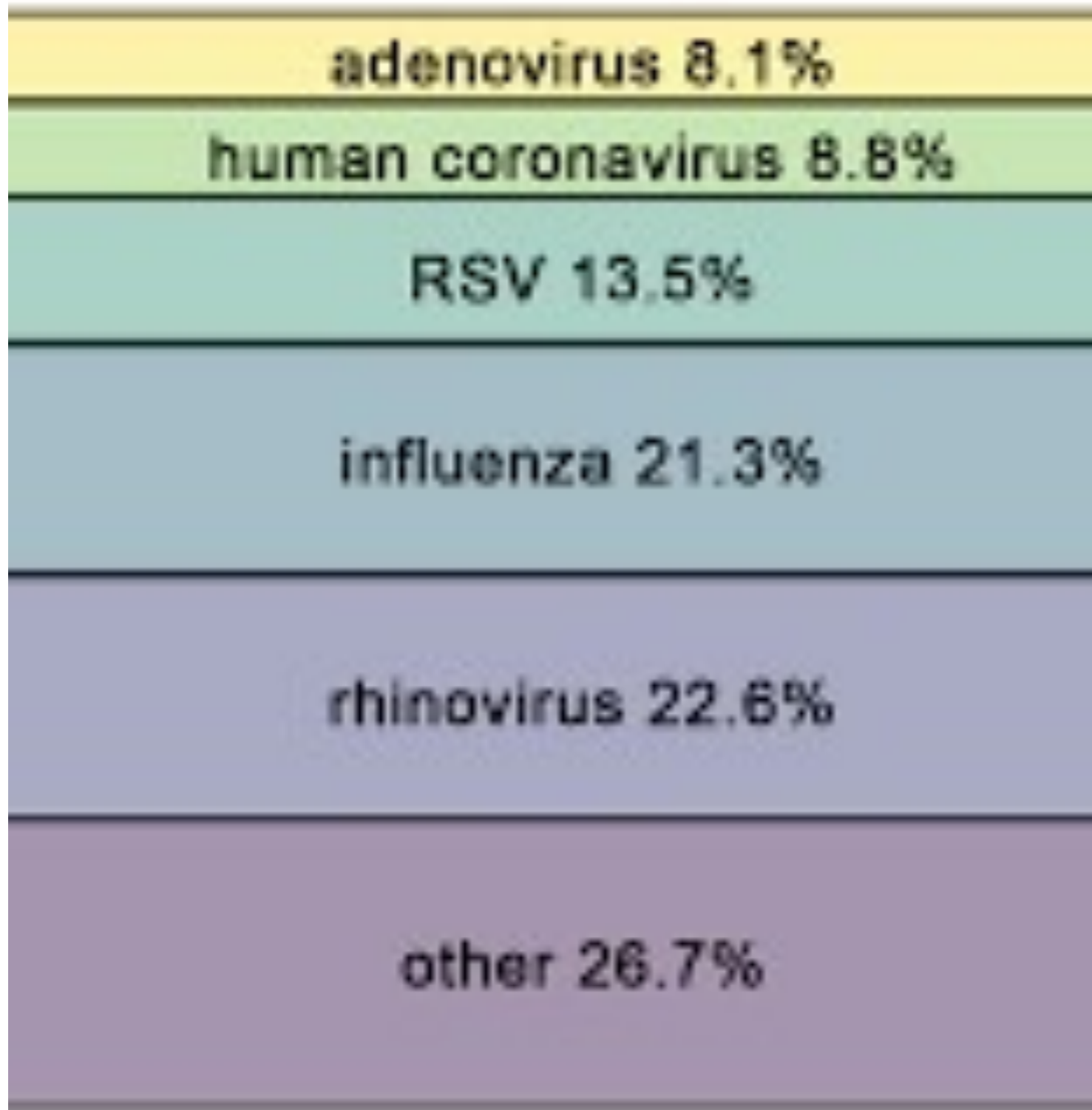
Viral Pathogen Contributions in Individuals with ILI
